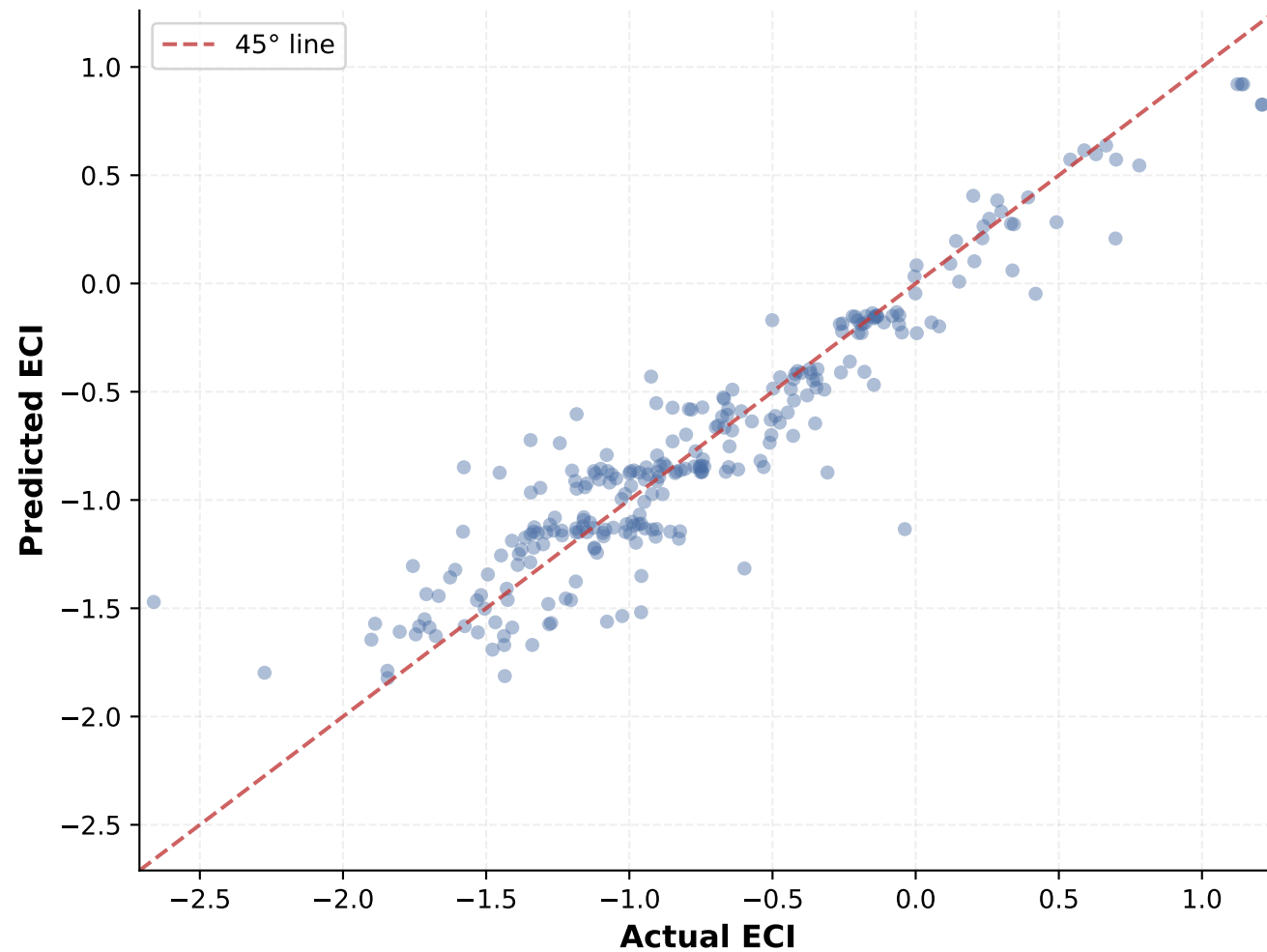
Random Forest — ECI | Test R^2=0.876 RMSE=0.2297
