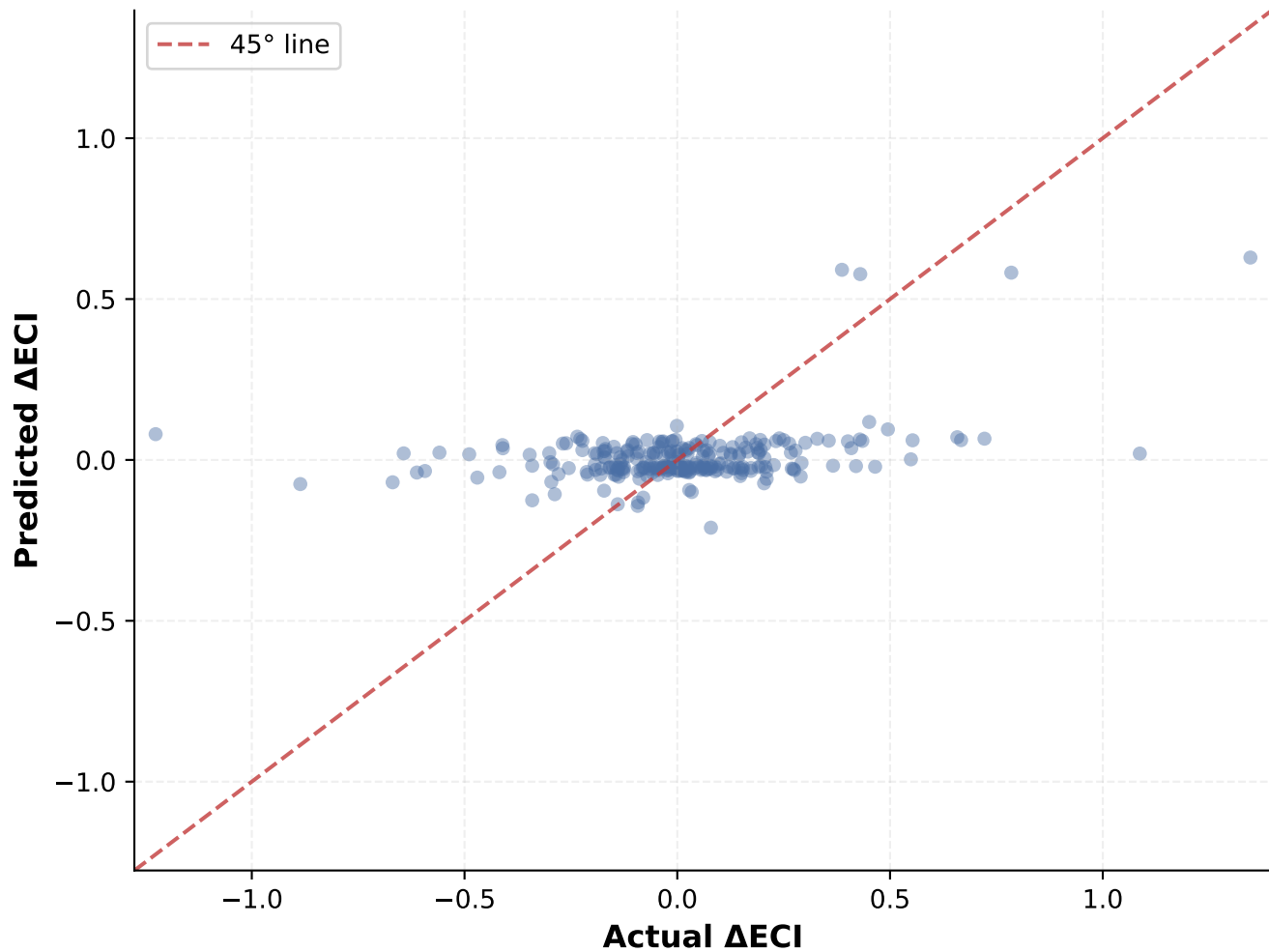
Random Forest — \Delta ECI | Test R^2=0.158 RMSE=0.2359
